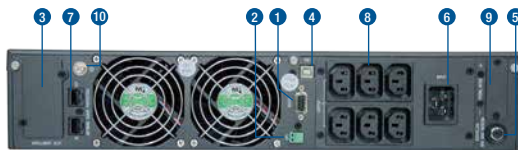
AP160i - 2KS rear panel
