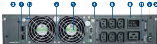
AP160i - 3KS rear panel
