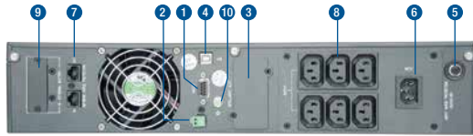
AP160i - 1K rear panel
