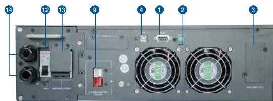
AP160i - 6KS & 10KS rear panel
